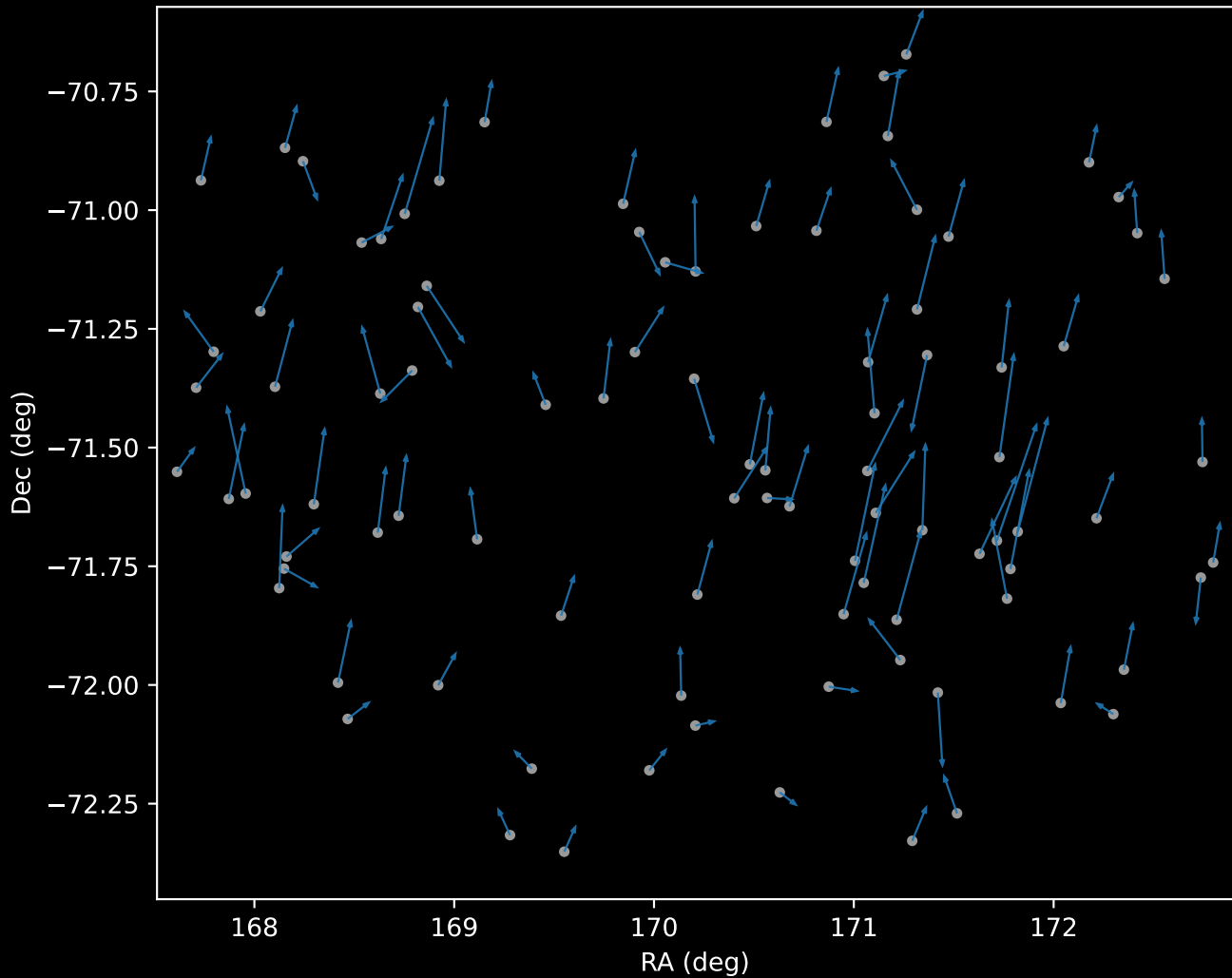
APOGEE DR17 Cluster 0 Proper Motion Vectors (n=94)
