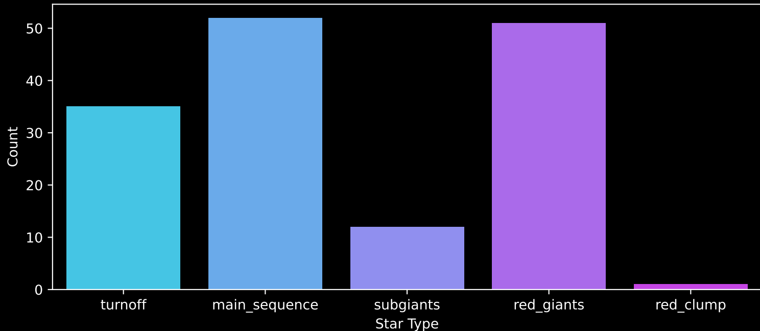
APOGEE DR17 Field: [284-36-O_TESS] Count plot of Star Type
