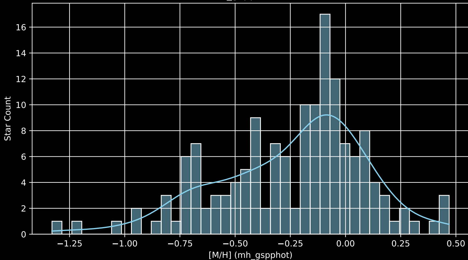
APOGEE DR17 Field: [284-36-O_TESS [M/H] (mh_gspphot) (n= 151)
