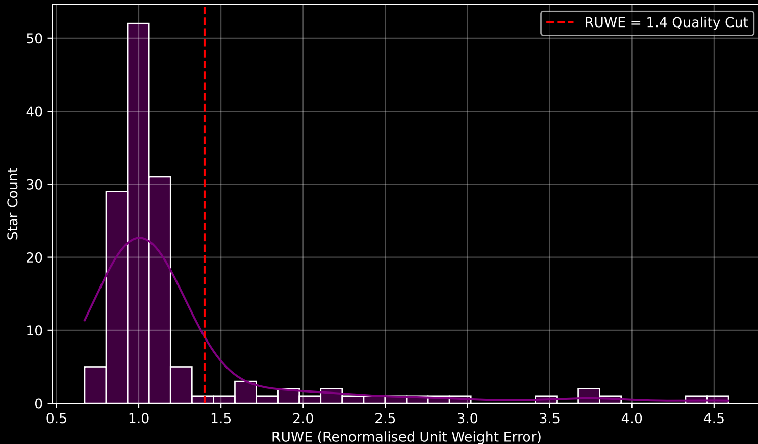
GAPOGEE DR17 Field [284-36-O_TESS] RUWE Distribution (n= 145)
