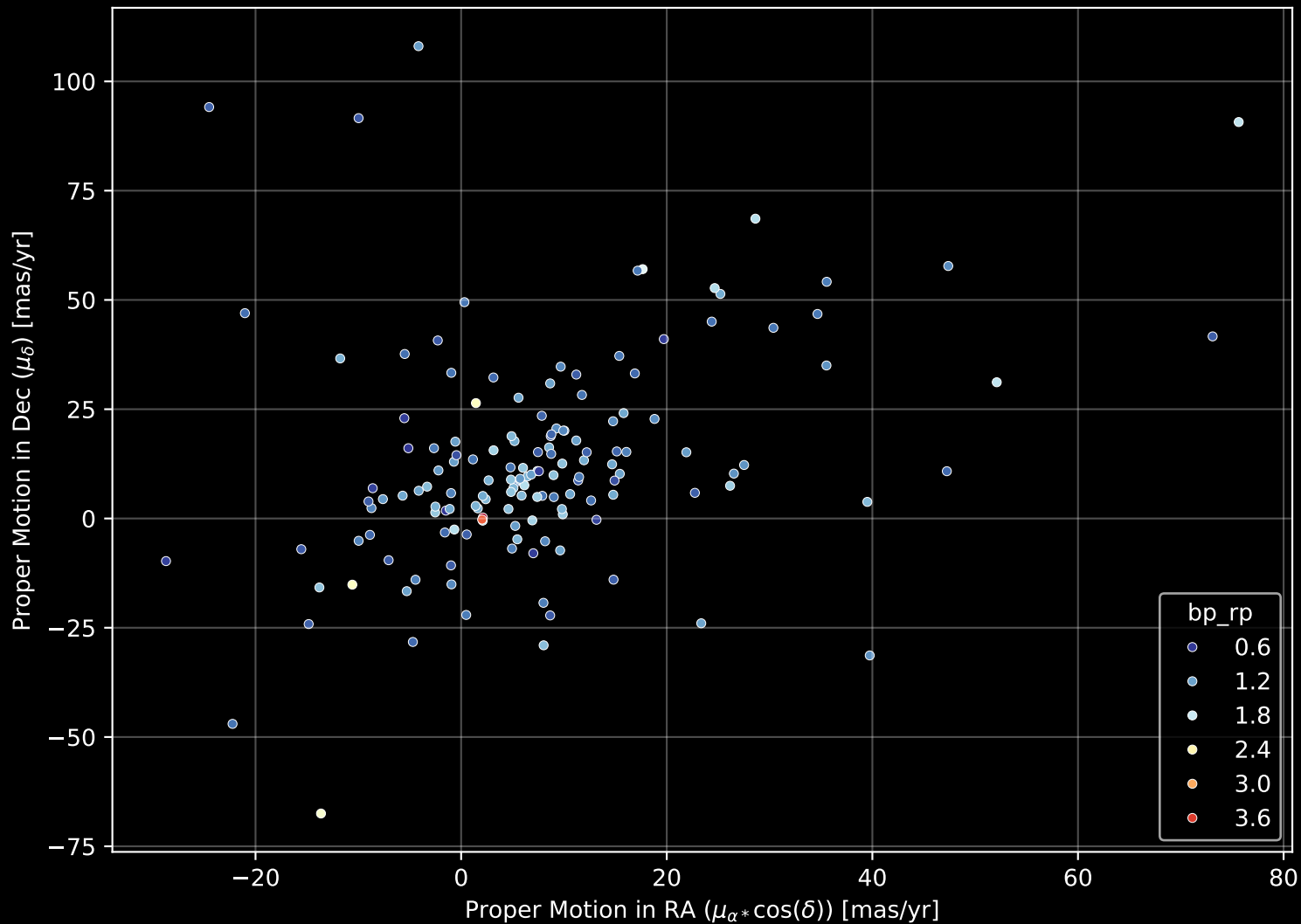
APOGEE DR17 Field: [284-36-O_TESS] Proper Motion Diagram (n= 151)
