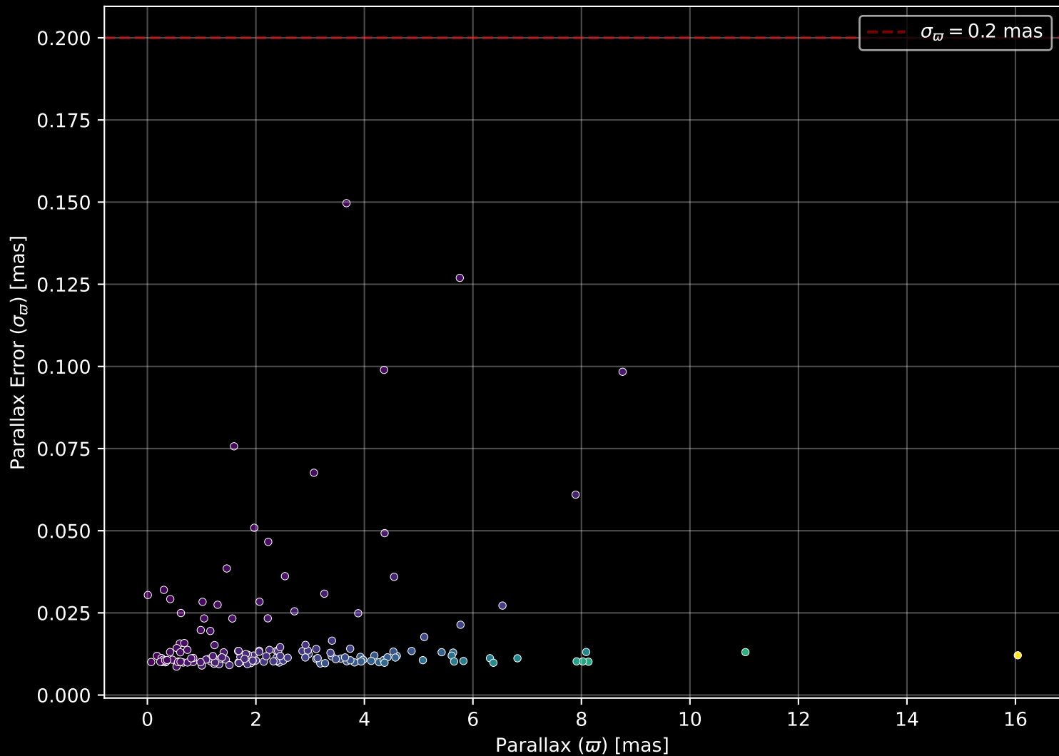
APOGEE DR17 Field: [284-36-O_TESS] Parallax Quality (n= 151)
